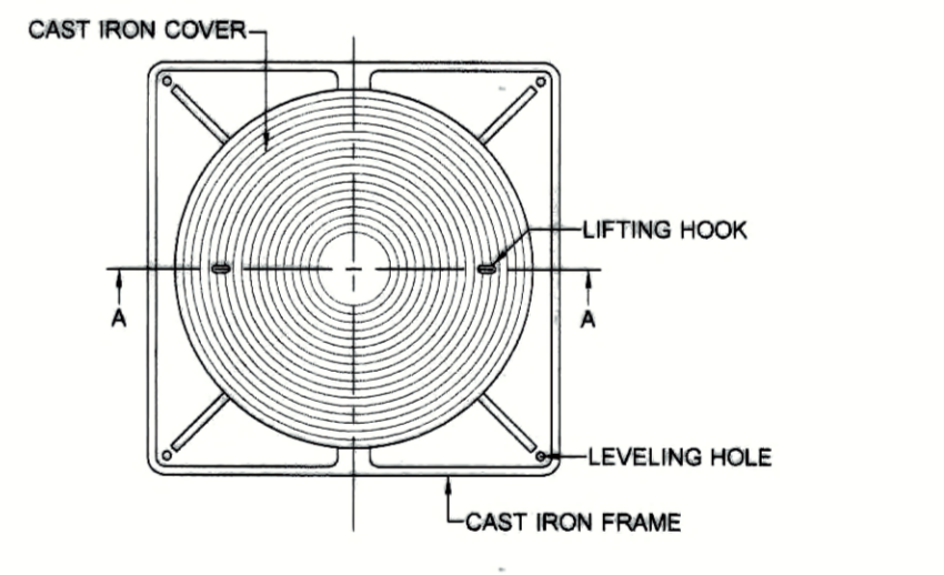
MANHOLE COVER DETAIL
