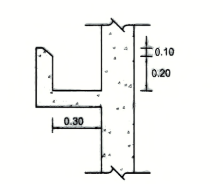
DETAIL OVERFLOW WEIR
